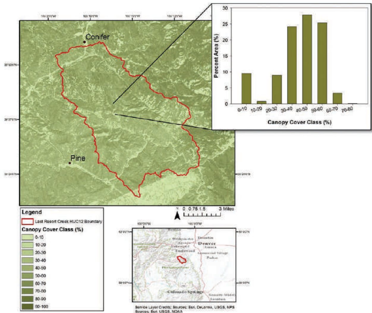
Figure 26 —Distribution of canopy cover classes within the Last Resort Creek subwatershed of the Upper South Platte watershed. Most of the area is in medium-density forest structures (40–70 percent canopy cover). The goal of restoration is to shift the distribution toward openings and low-density forest structures where ecologically appropriate, as well as retain some high-density forest structures because they are also underrepresented.
