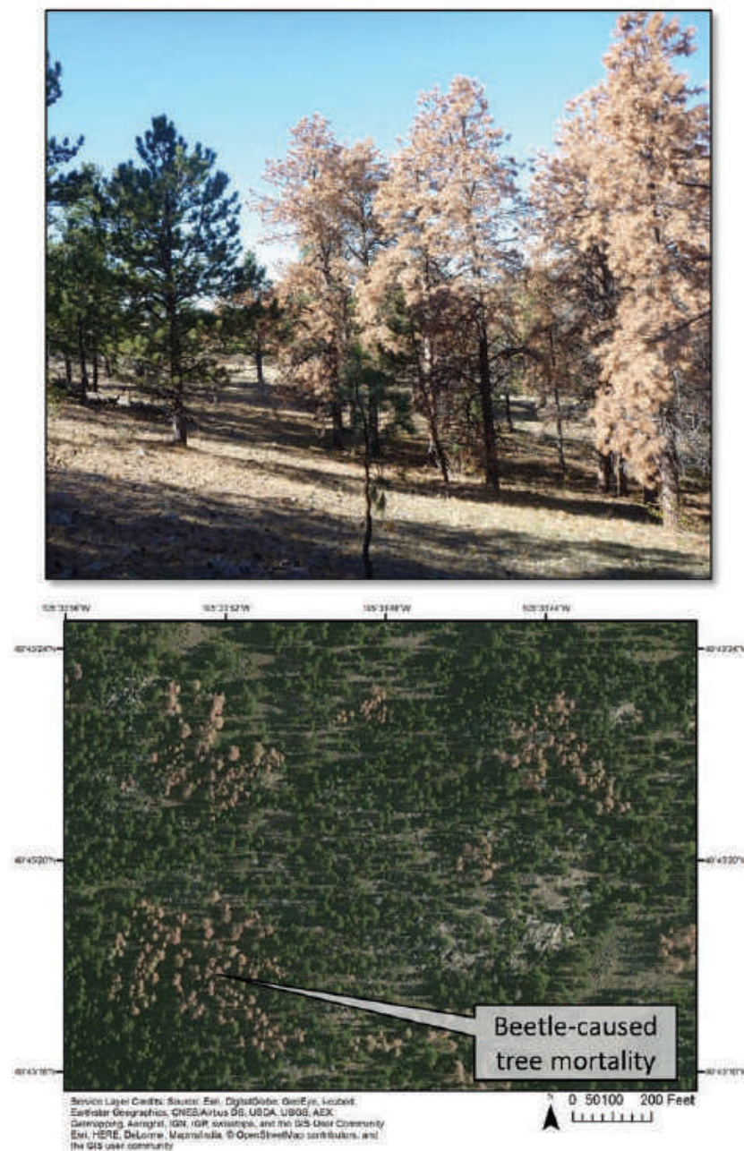
Figure 21 —(a) Ponderosa pine tree mortality as a result of mountain pine beetle in Larimer County, Colorado (photo by J. Briggs, U.S. Geological Survey); (b) aerial image of 1- to 3-acre patches of beetle-caused mortality in Larimer County. Mountain pine beetle often kills trees in groups, thereby creating openings for understory vegetation development and tree regeneration.
