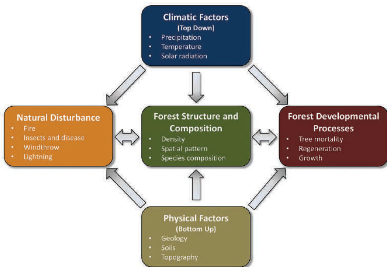
Figure 8 —Generalized conceptual model illustrating interactions among climate, natural disturbance, forest developmental processes, and physical factors that influence forest structure and composition on the Front Range.
